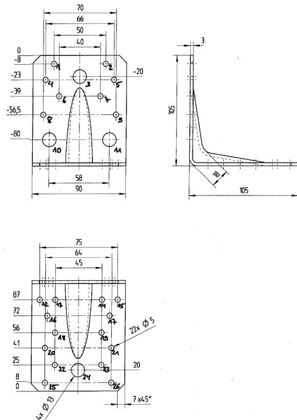
Figure A.16 Dimensions of AB 8633 10 FH1
