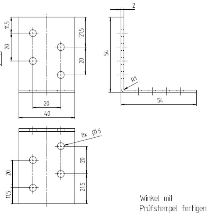
Figure A.6 Dimensions of Angle Bracket 8620
