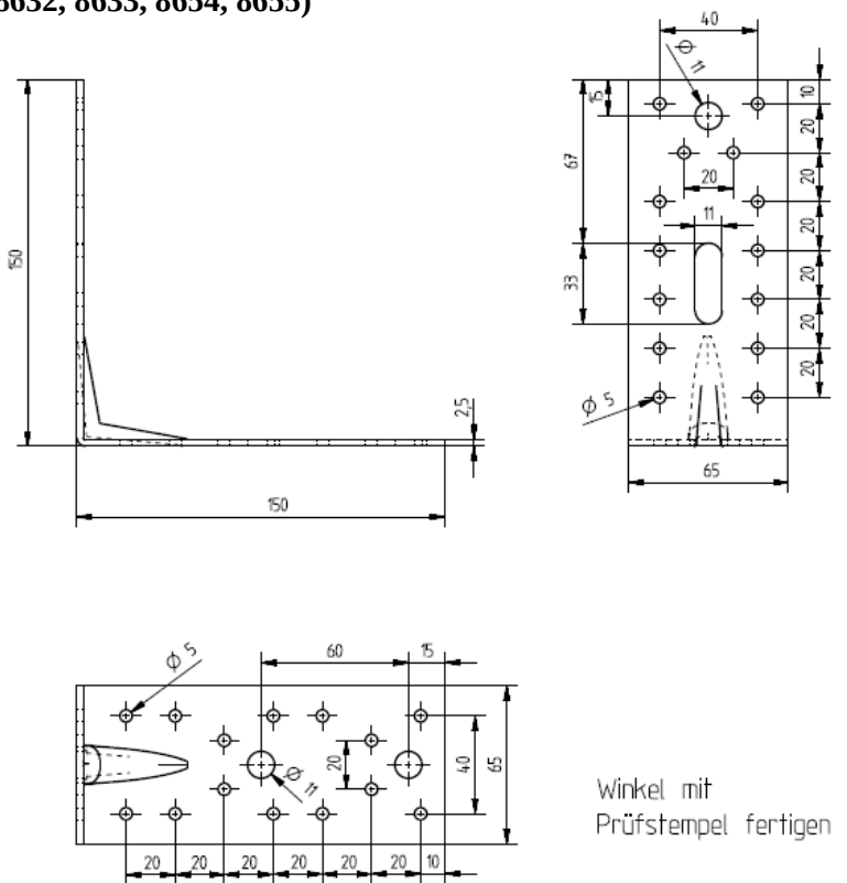
Figure A.23 Dimensions of Angle Bracket 8628
