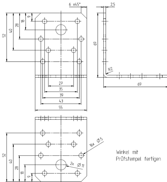
Figure A.9 Dimensions of Angle Bracket 8624
