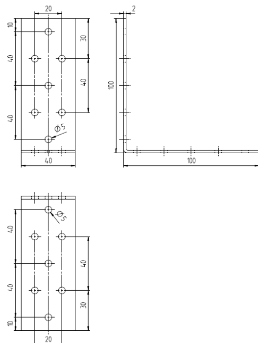
Figure A.4 Dimensions of Angle Bracket 8615
