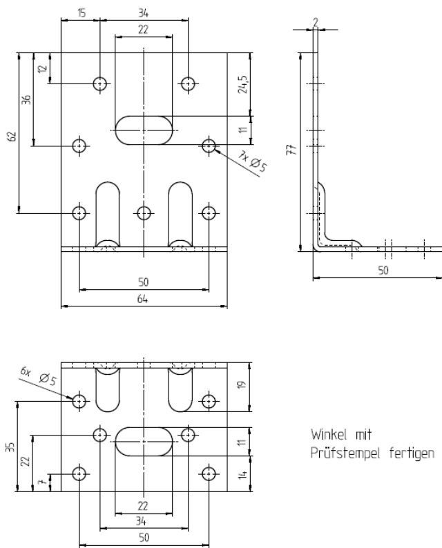
Figure A.24 Dimensions of Angle Bracket 8629
