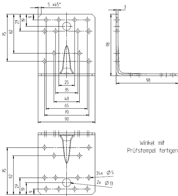
Figure A.26 Dimensions of Angle Bracket 8633
