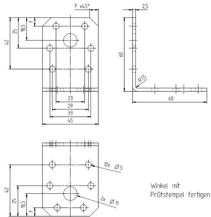
Figure A.12 Dimensions of Angle Bracket 8627
