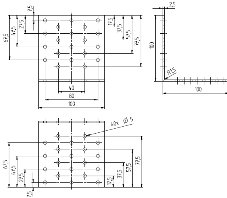
Figure A.21 Dimensions of Angle Bracket 8645
