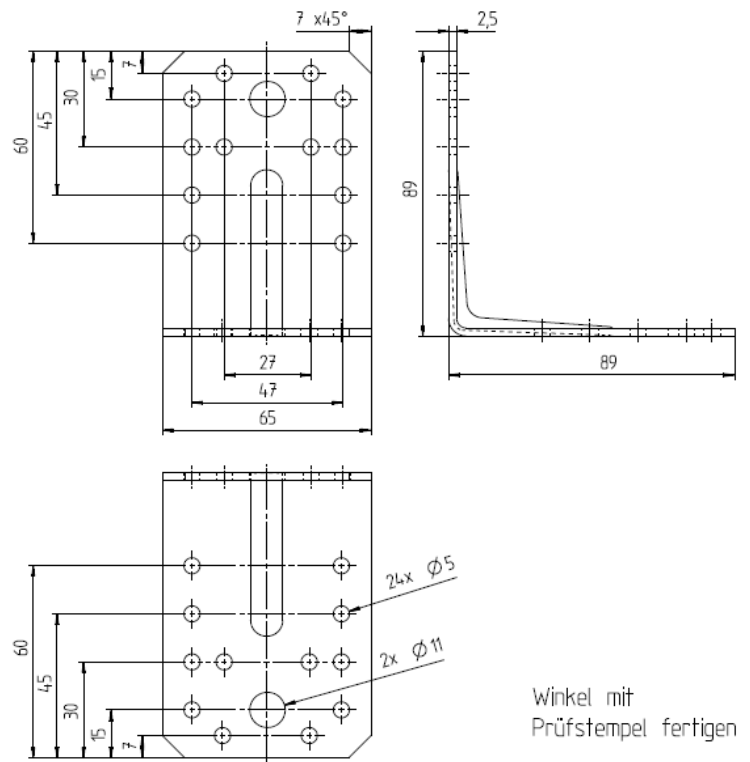
Figure A.25 Dimensions of Angle Bracket 8632
