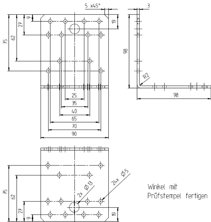
Figure A.11 Dimensions of Angle Bracket 8626
