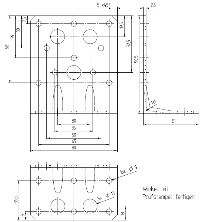
Figure A.27 Dimensions of Angle Bracket 8654
