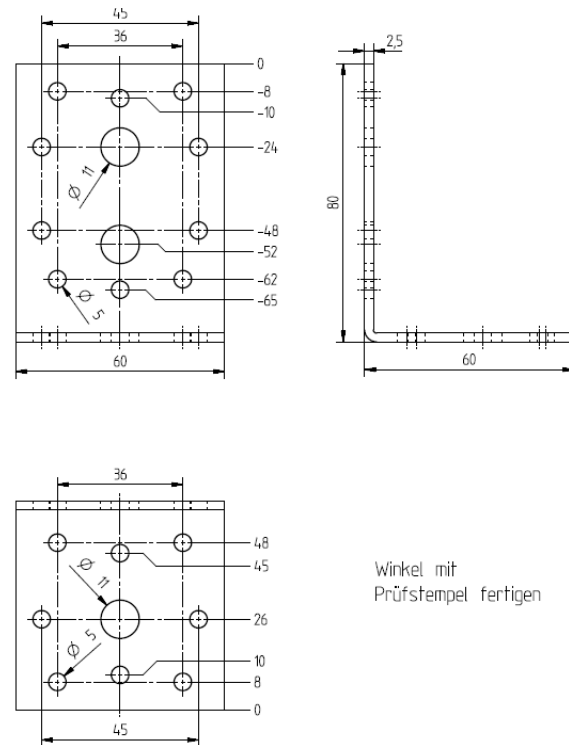
Figure A.2 Dimensions of Angle Bracket 8613
