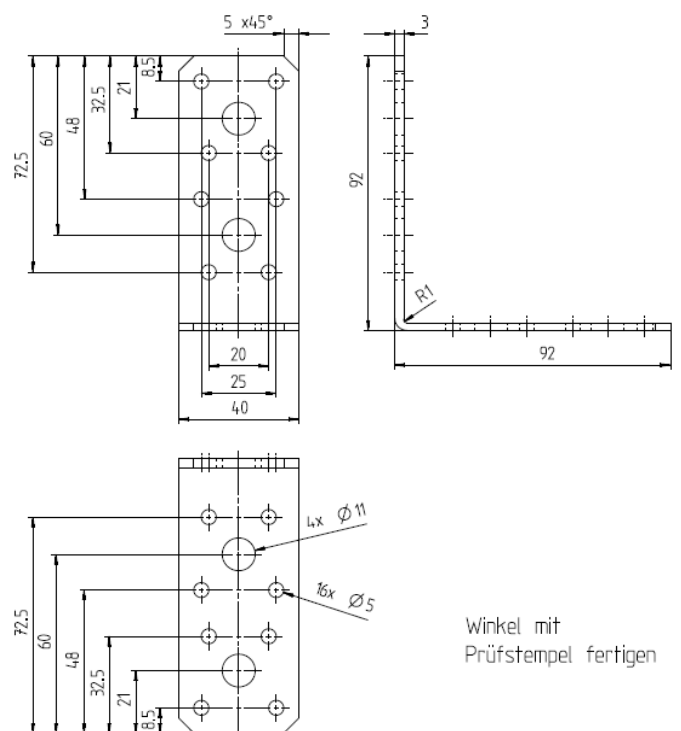
Figure A.8 Dimensions of Angle Bracket 8623
