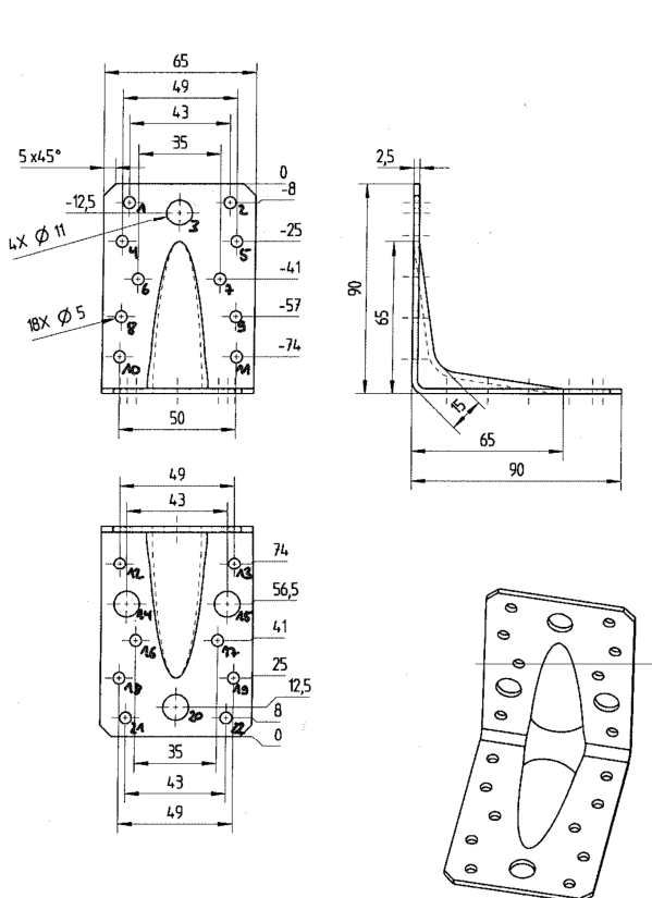
Figure A.15 Dimensions of AB 8632 90 FH1
