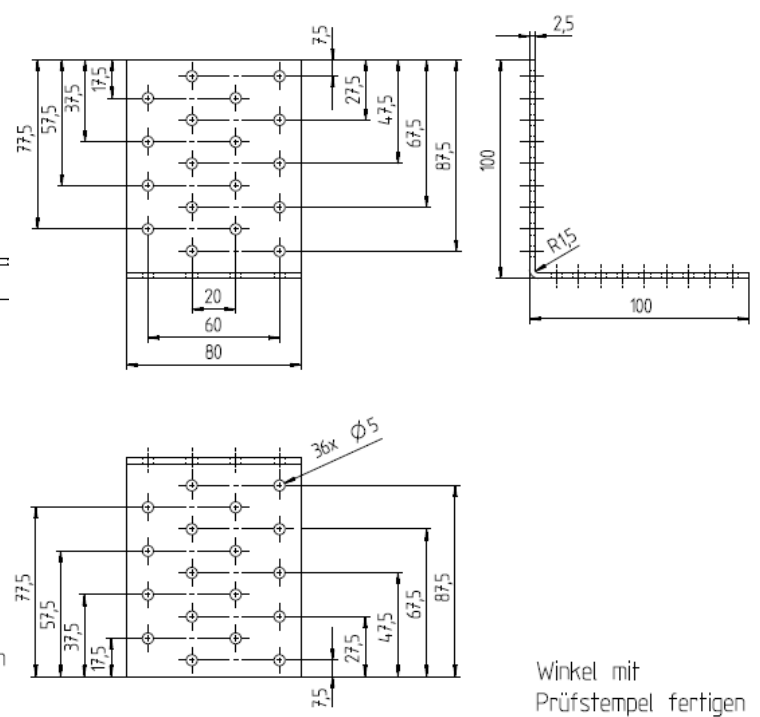
Figure A.20 Dimensions of Angle Bracket 8644
