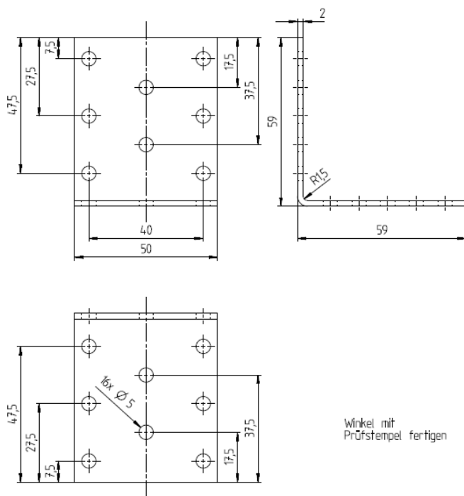
Figure A.15 Dimensions of Angle Bracket 8636
