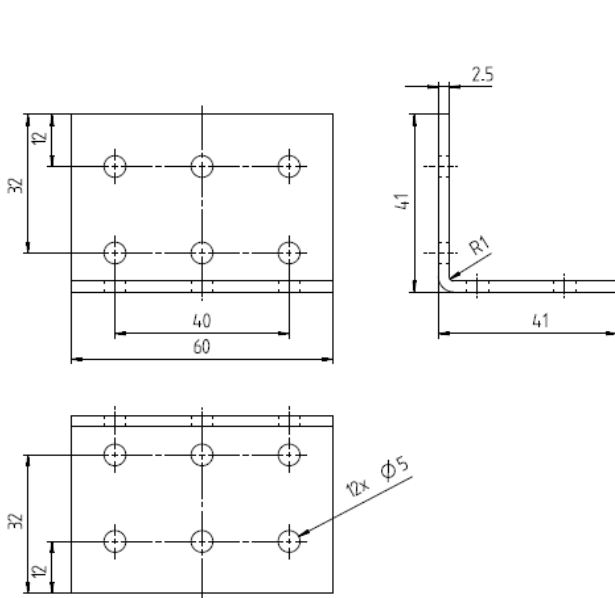
Figure A.13 Dimensions of Angle Bracket 8634
