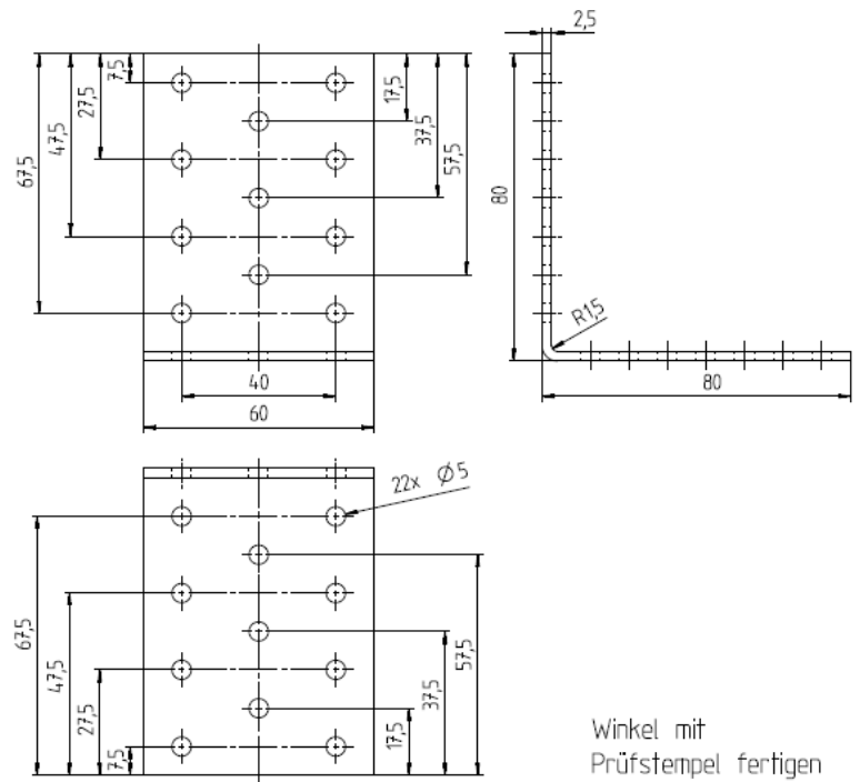
Figure A.18 Dimensions of Angle Bracket 8640
