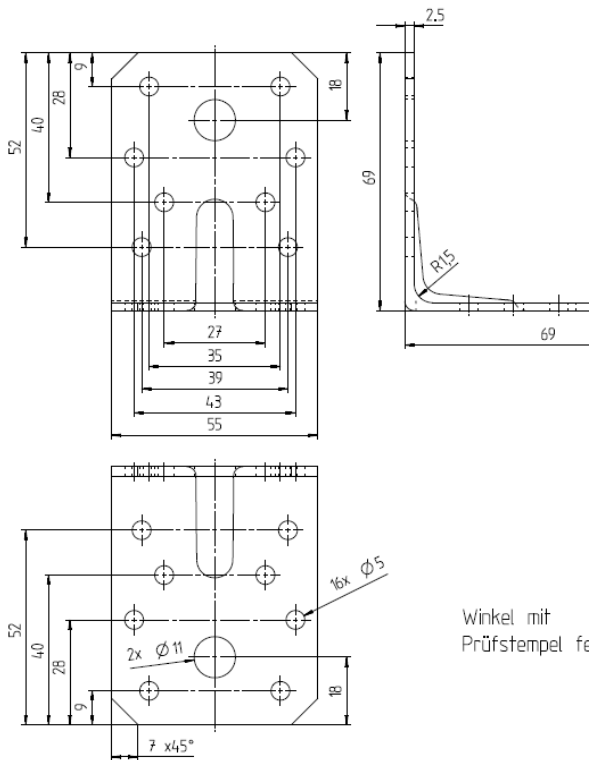
Figure A.22 Dimensions of Angle Bracket 8622
