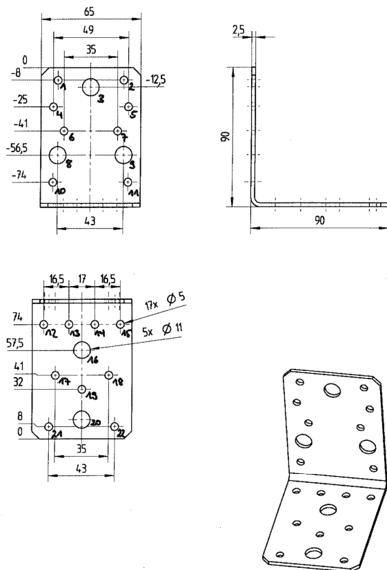
Figure A.13 Dimensions of AB 8625 90 FH1
