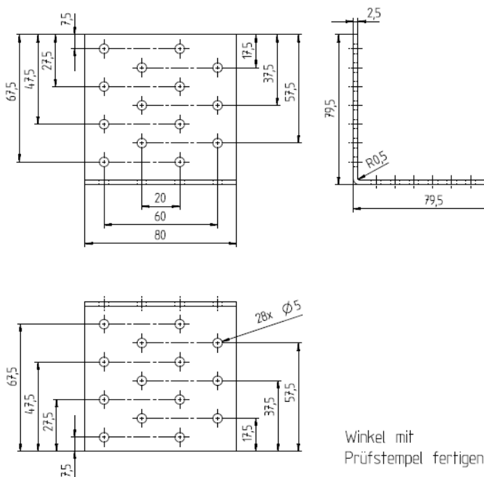
Figure A.19 Dimensions of Angle Bracket 8641
