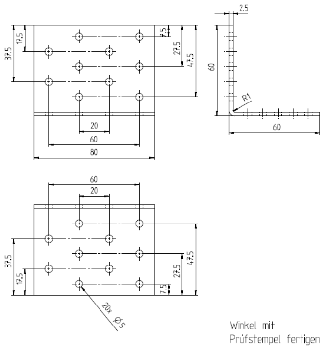
Figure A.17 Dimensions of Angle Bracket 8638
