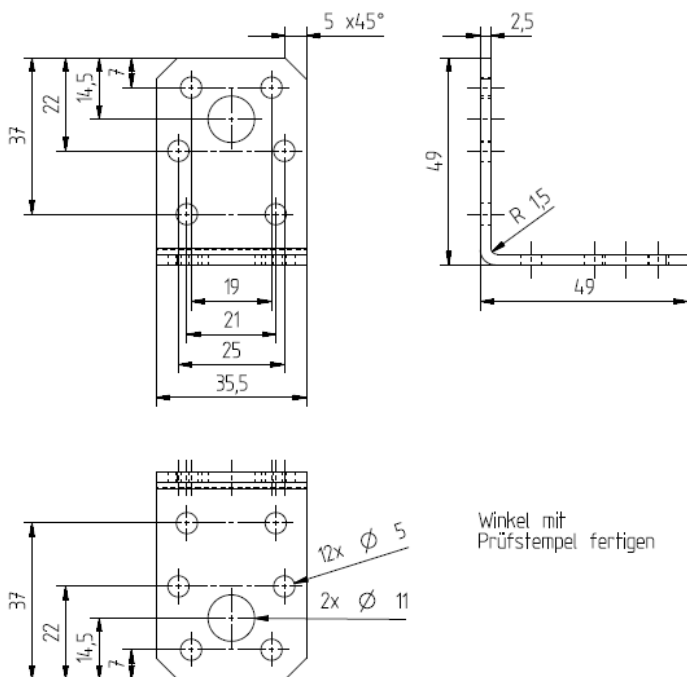
Figure A.5 Dimensions of Angle Bracket 8617
