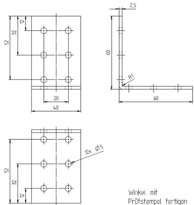
Figure A.14 Dimensions of Angle Bracket 8635
