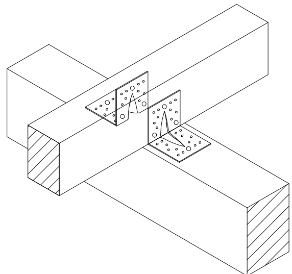
Figure A.29 Typical installation
