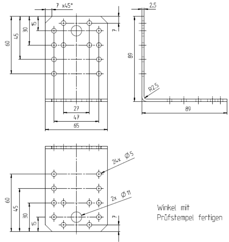
Figure A.10 Dimensions of Angle Bracket 8625
