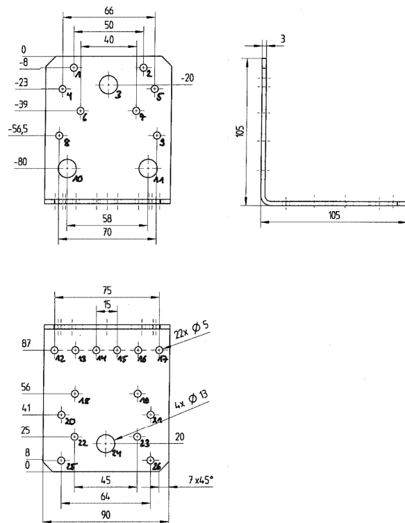
Figure A.14 Dimensions of AB 8626 10 FH1
