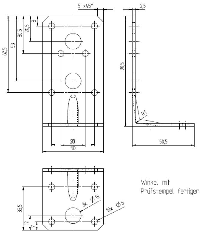
Figure A.28 Dimensions of Angle Bracket 8655
