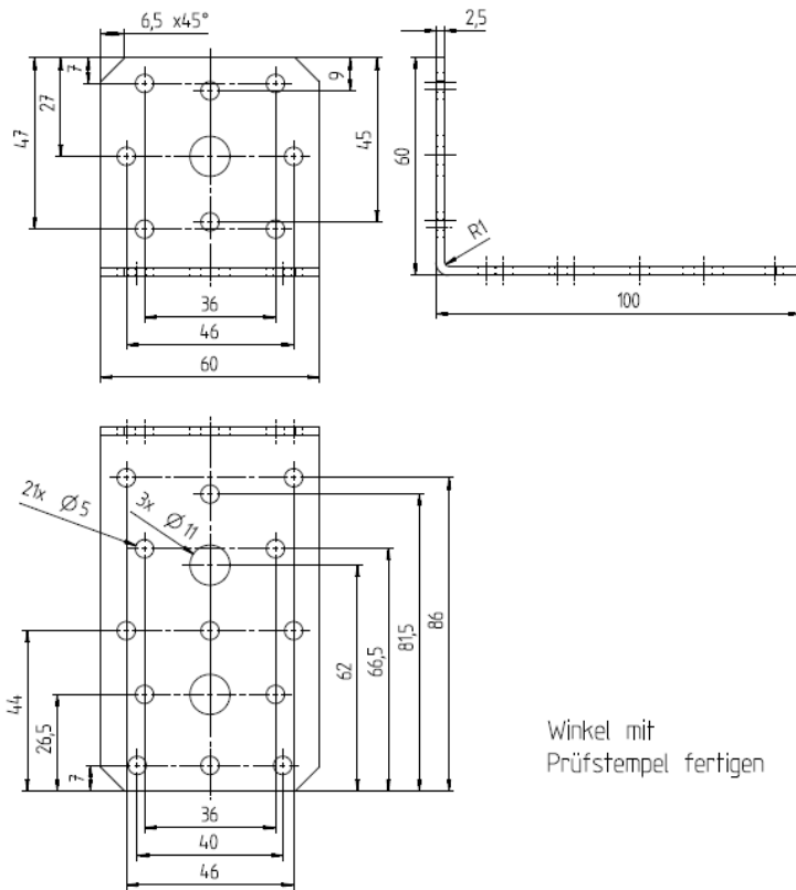
Figure A.5 Dimensions of Angle Bracket 8617
