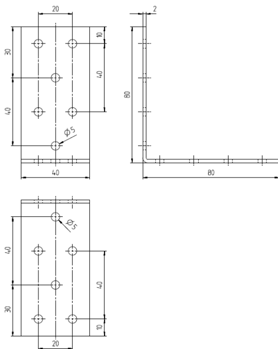
Figure A.3 Dimensions of Angle Bracket 8614
